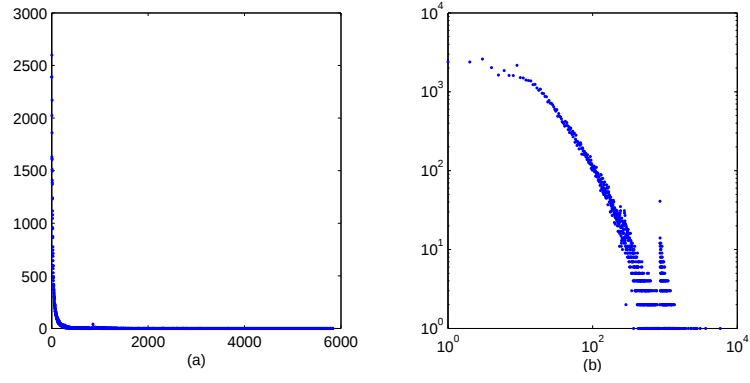
Figure 1: Distribution of the degree sequence of the cross-post graph in (a) linear (b) log-log scale
