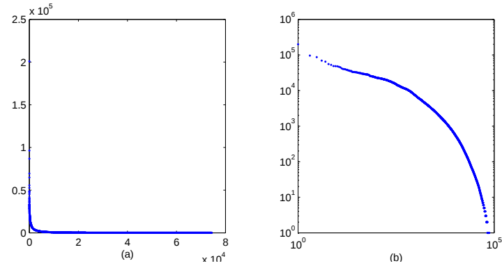
Figure 2: Distribution of the number of authors in (a) linear (b) log-log scale
