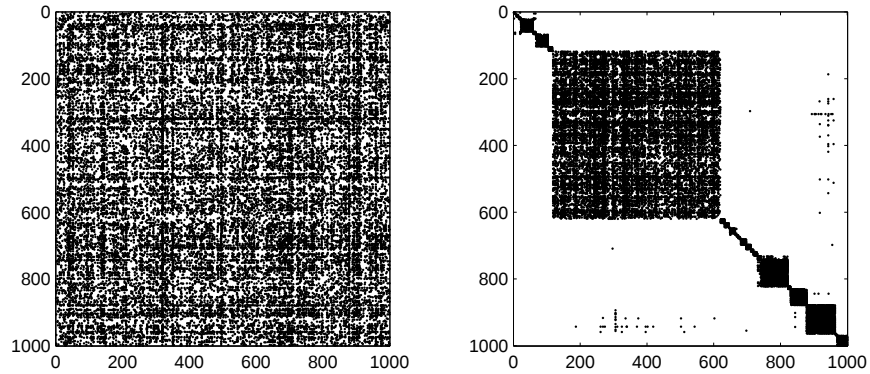
Figure 3: (a) The cross-post matrix restricted on the first one thousand newsgroups: a black point in position i and j indicates at least one cross-post between newsgroups i and j (b): The same matrix after reordering the newsgroup based on the result of our clustering. Note that the upper-right and lower-left of our matrix is now almost empty.
